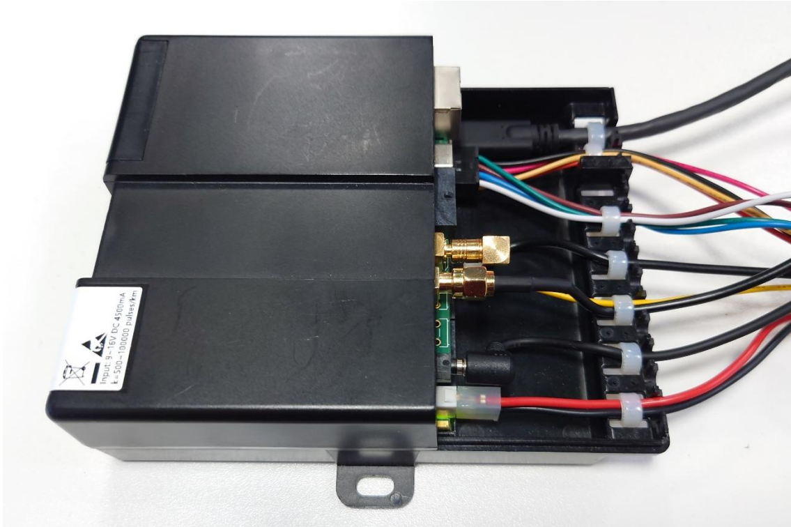
Figure 4.7 Secured cables
